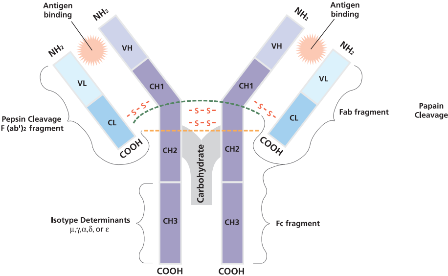
Figure 1. Basic Immunoglobulin Structure
